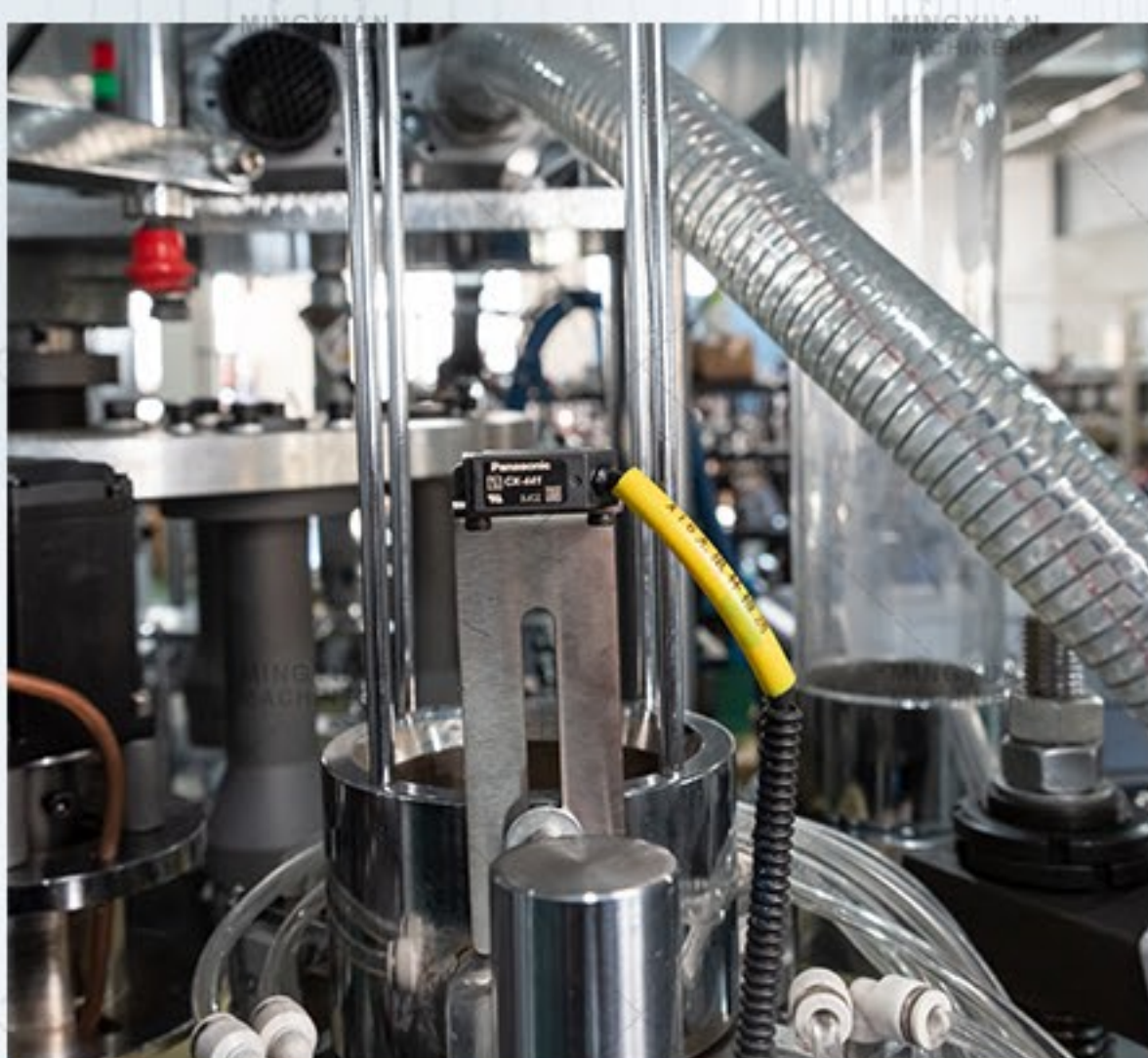
Paperless cup testing
