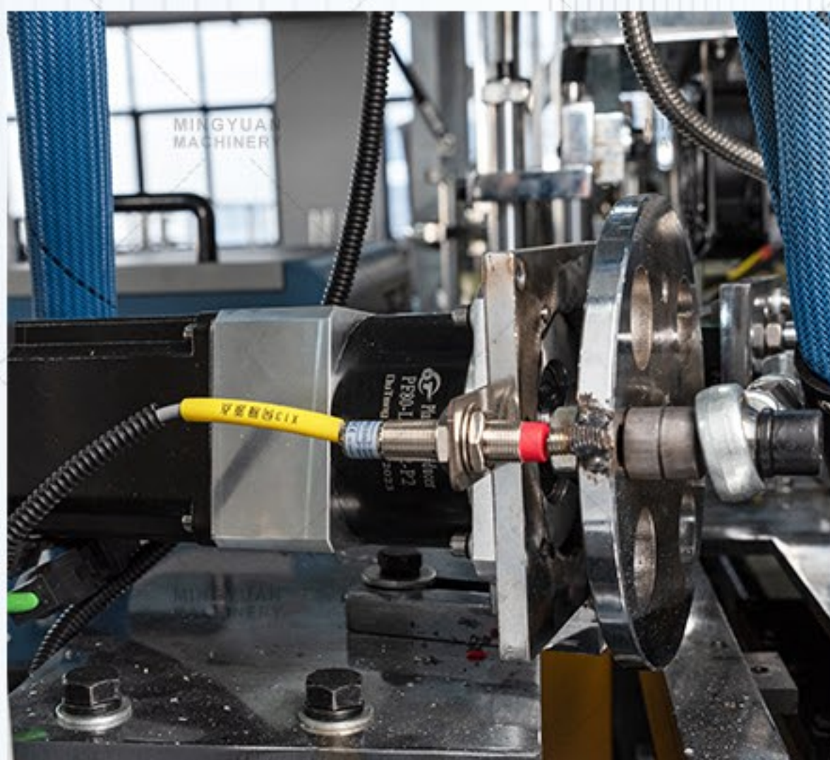
Servo origin
