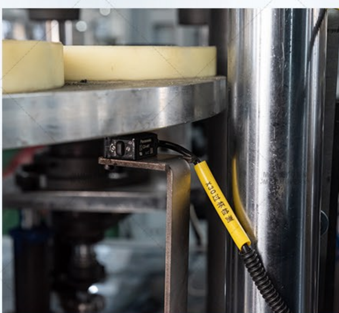
Over-cup detection
