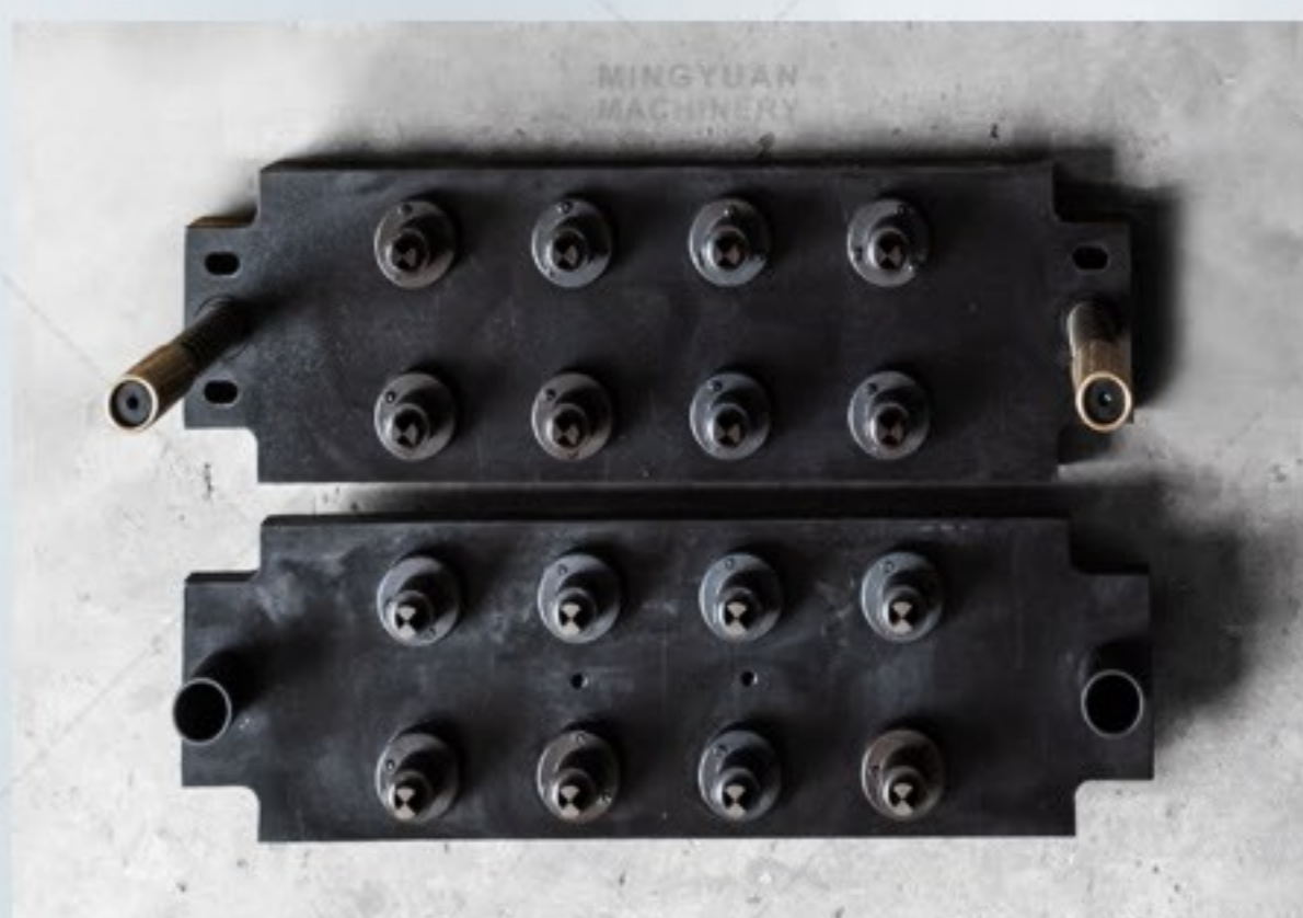
PUNCHING HOLE MOULD
